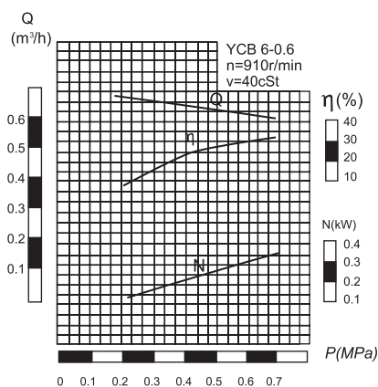
YCB 6-0.6 Diagram of performance Curve of Model YCB 6-0.6 Gear pump
