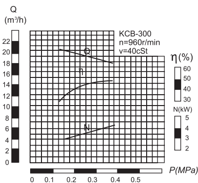
KCB-300 Diagram of performance Curve of Model KCB-300 Gear pump
