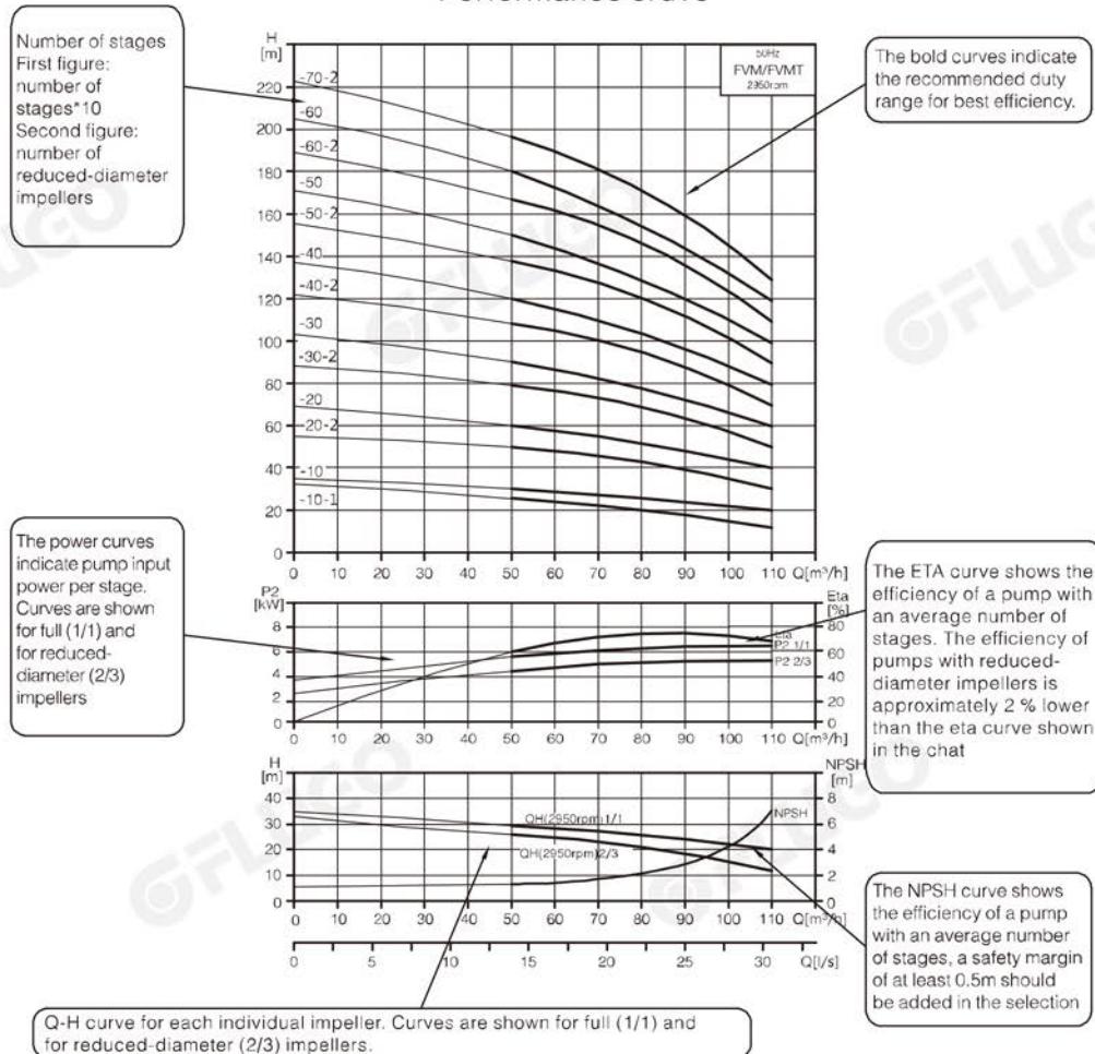
Performance cruve
