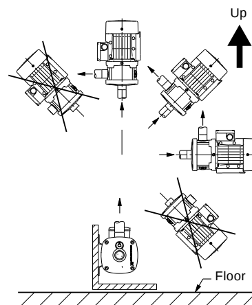
Fig. 10 Pump positions
