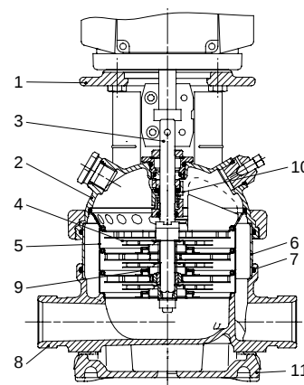
Sectional drawing
