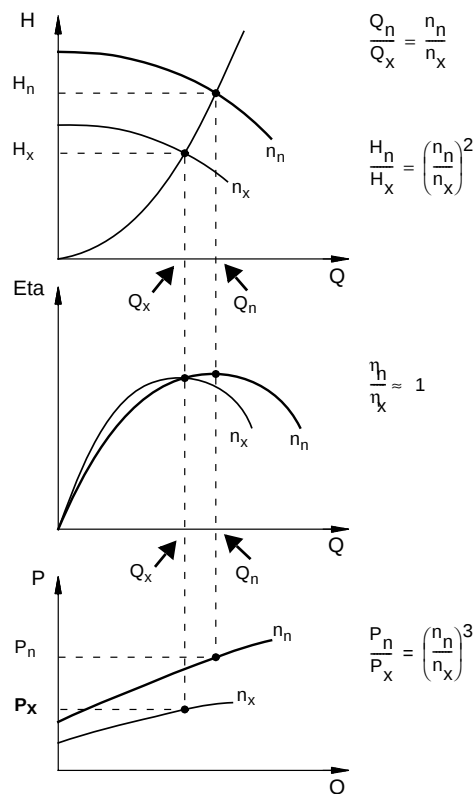
Fig. 20 Affinity equations
