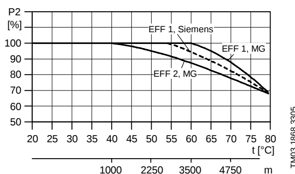
Fig. 5 Motor output depends on temperature/altitude
