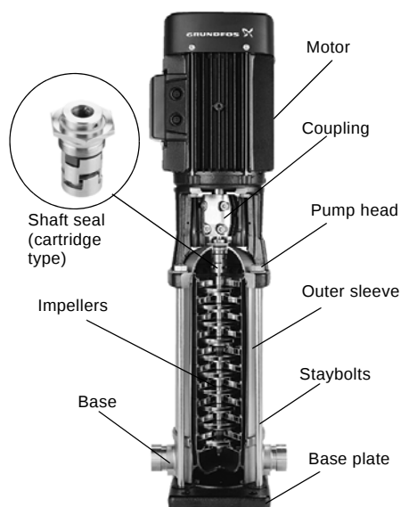
Fig. 3 CR pump
