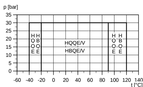
Fig. 14 Operating range of standard shaft seals
