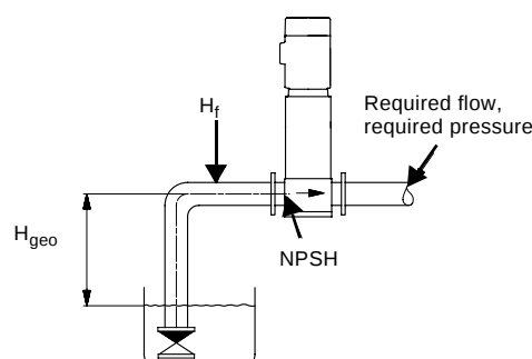
Fig. 18 Dimensional data
