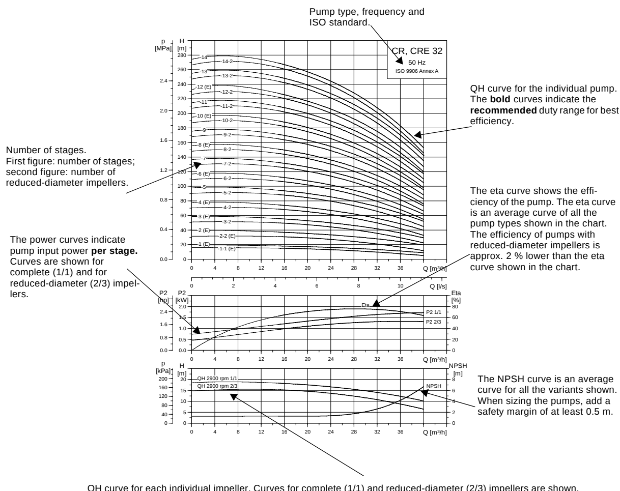
Fig. 26 How to read the curve charts
