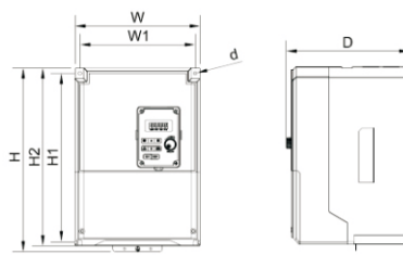
(Figure B) 380V: 10~20HP (IP20)
